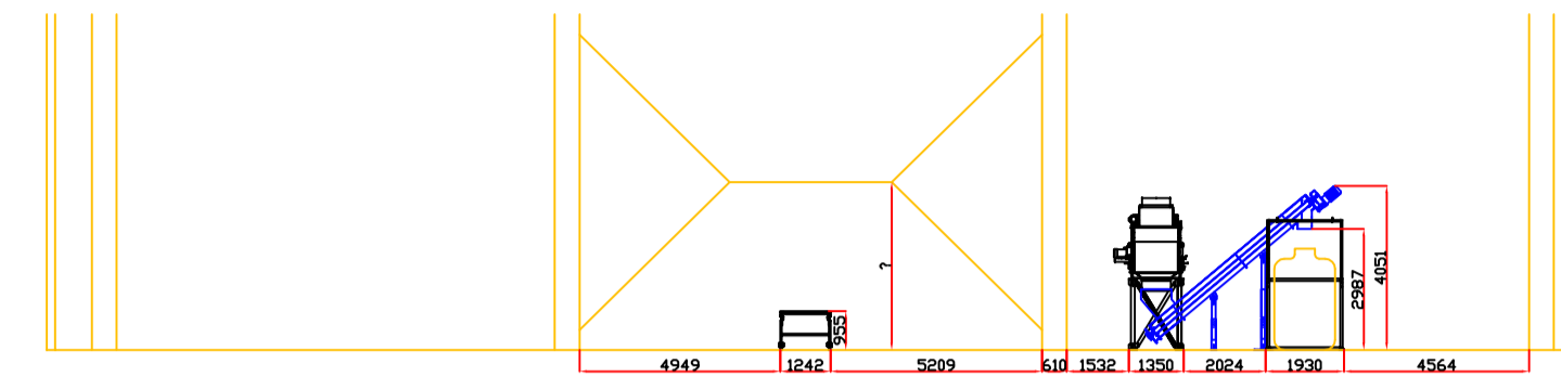
VIEW E
